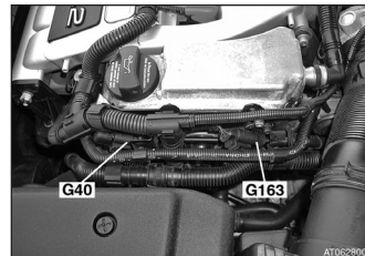
Location of ignition components on 3.2L engine. 28 Ignition System
