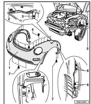
Detailed exploded views including front body assembly.
