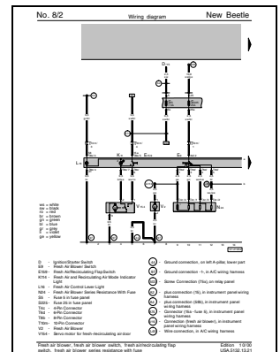
Up-to-date factory issued electrical wiring diagrams.
